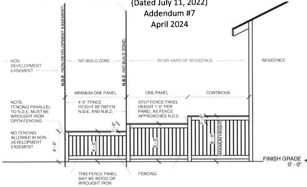
1 SIDE VIEW AT FENCING
