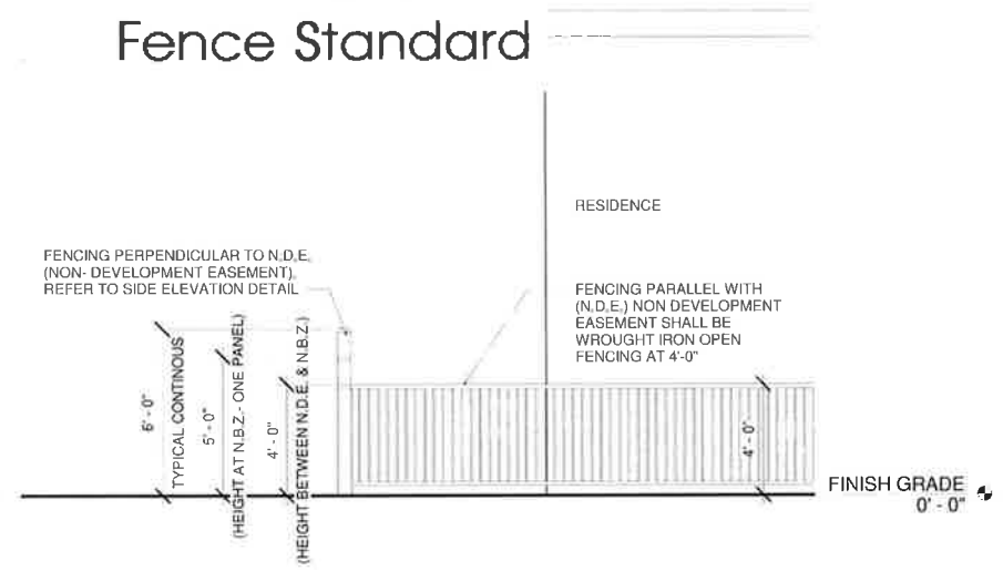
2 REAR VIEW AT FENCING AT N.D.E.
